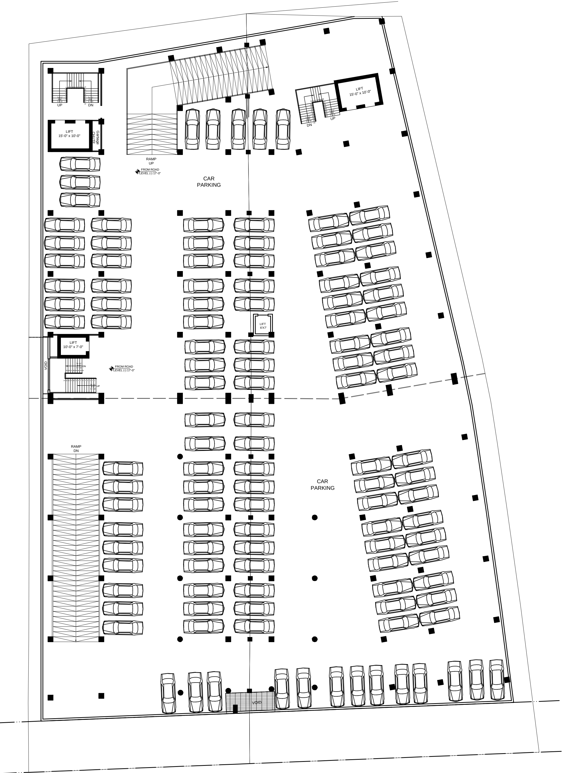
FIRST BASEMENT PLAN
